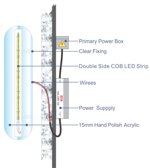
*Section Details
