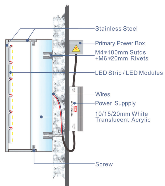
*Section Details
