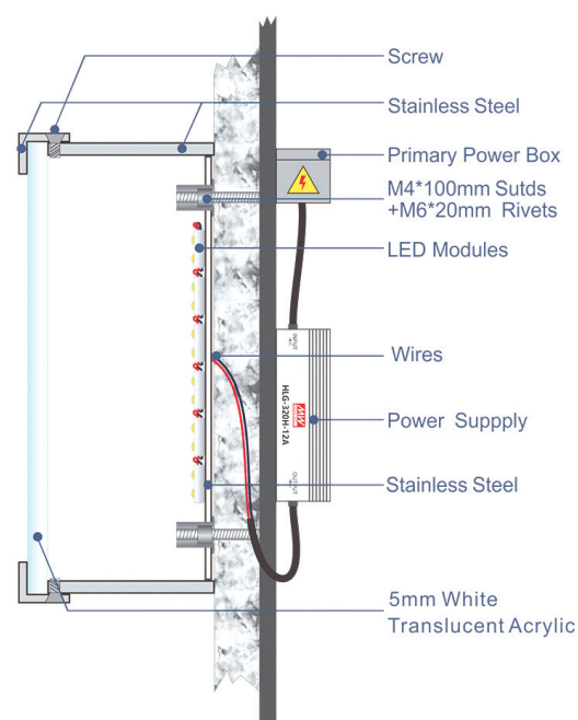
*Section Details
