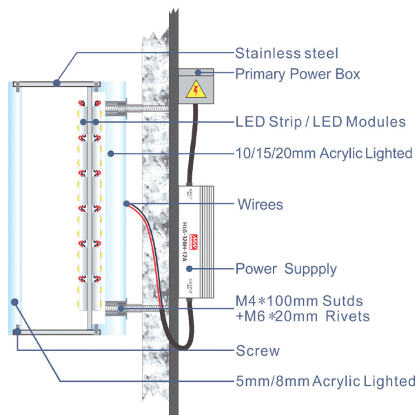
*Section Details
