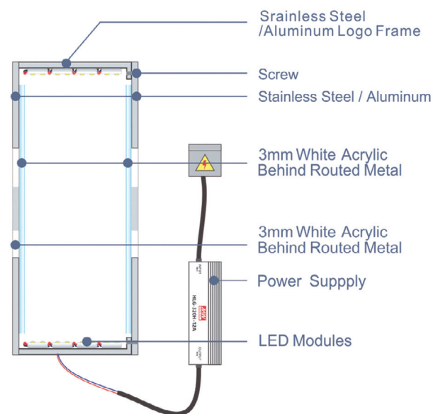
*Section Details
