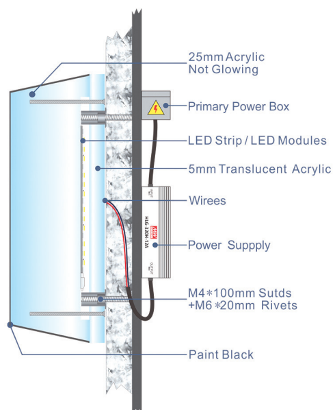
*Section Details
