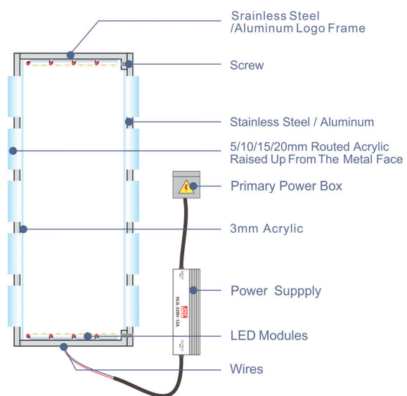
*Section Details
