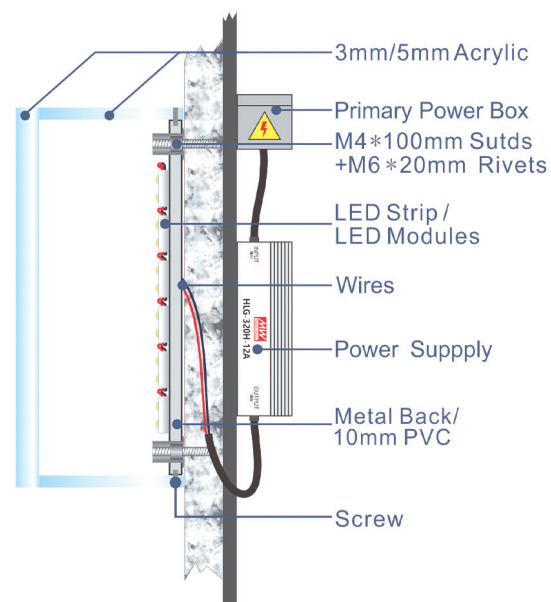
*Section Details
