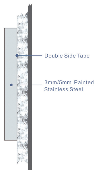
*Section Details
