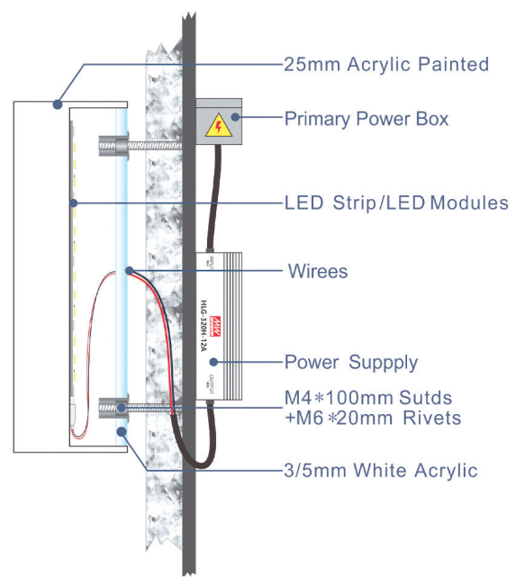
*Section Details
