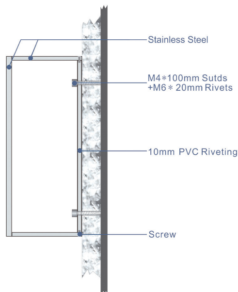
*Section Details
