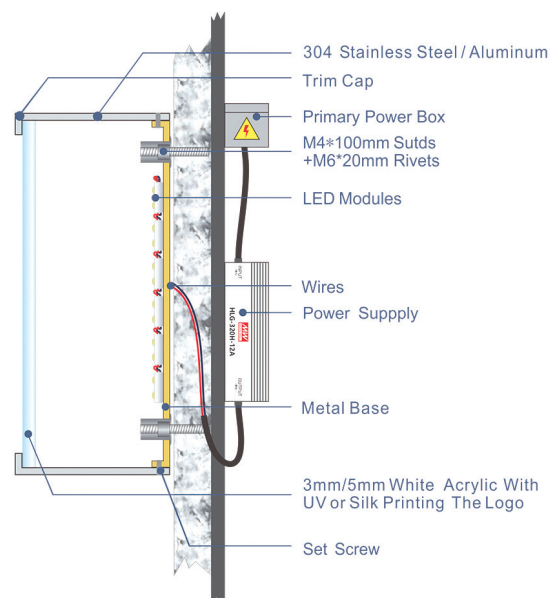
*Section Details
