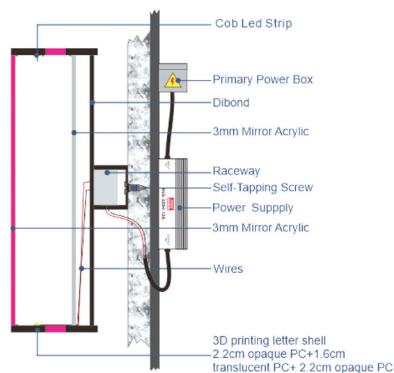
*Section Details
