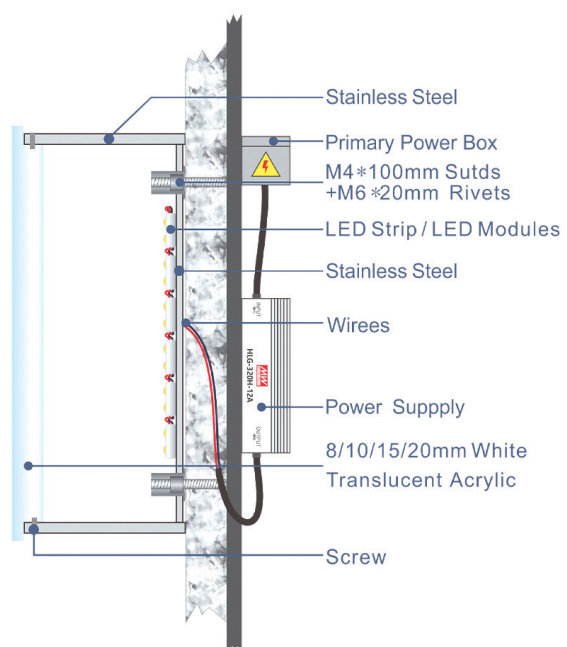
*Section Details
