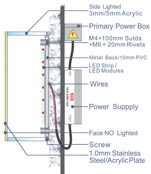
*Section Details
