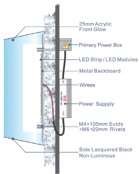
*Section Details
