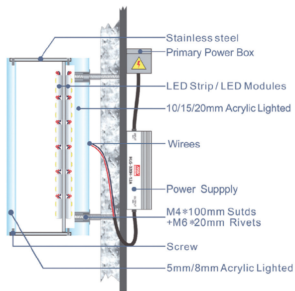
*Section Details
