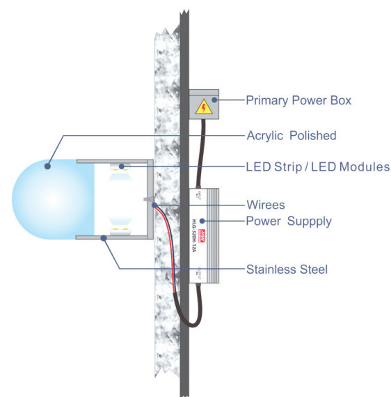
*Section Details
